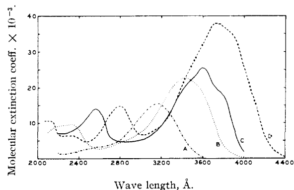
Fig. 2.—Ultraviolet absorption spectra of some aldehyde derivatives of the tetramer of increasing unsaturation: A, - · - · - ·, isobutylidene derivative; B, . . . . ., allylidene derivative; C, ———, benzylidene derivative; D, - - - - -, cinnamylidene derivative.
