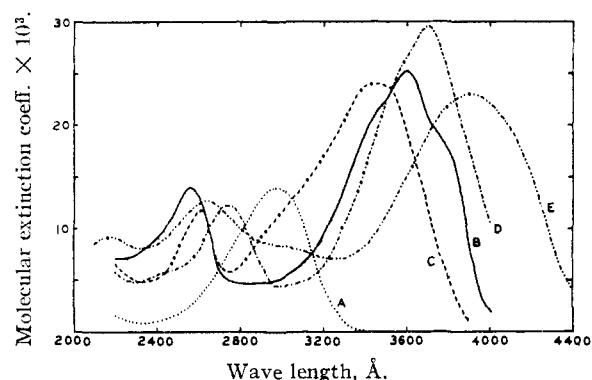
Fig. 3.—Ultraviolet absorption spectra of the tetramer and its aryl aldehyde derivatives: A, . . . . ., tetramer; B, ———, benzylidene derivative; C, - - - - -, benzylidene-acetyl derivative; D, - · - · - ·, p -hydroxybenzylidene derivative; E, - - - - -, p -nitrobenzylidene derivative.
